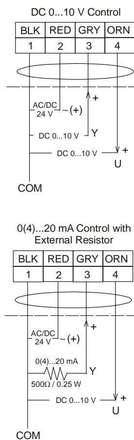
Figure 10: Control Wiring Diagrams
