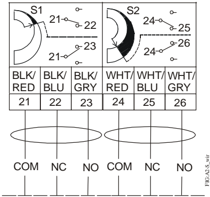
Figure 9: Auxiliary Switch Wiring Diagram for ES177A2-S Models
