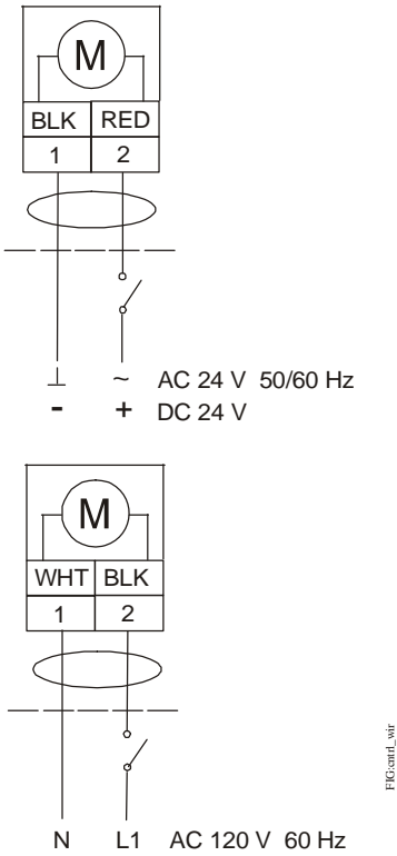
Figure 10: Control Wiring Diagrams
