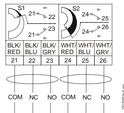
Figure 9: Auxiliary Switch Wiring Diagram for ES89Ax-S Series Models
