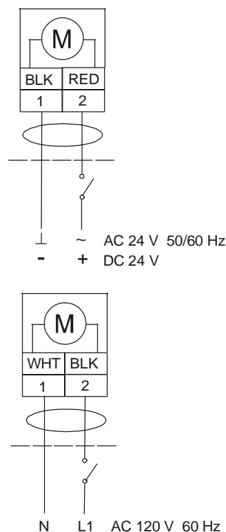
Figure 10: Control Wiring Diagrams
