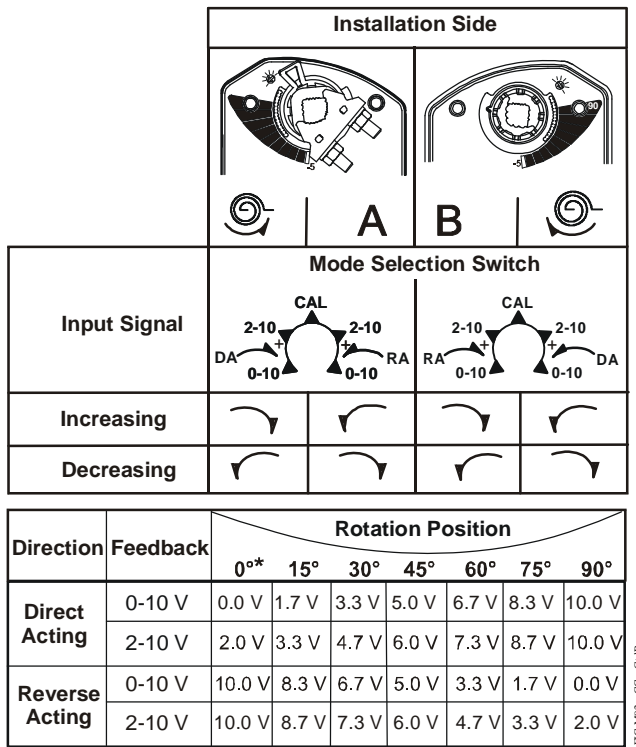
Figure 13: Control Response
