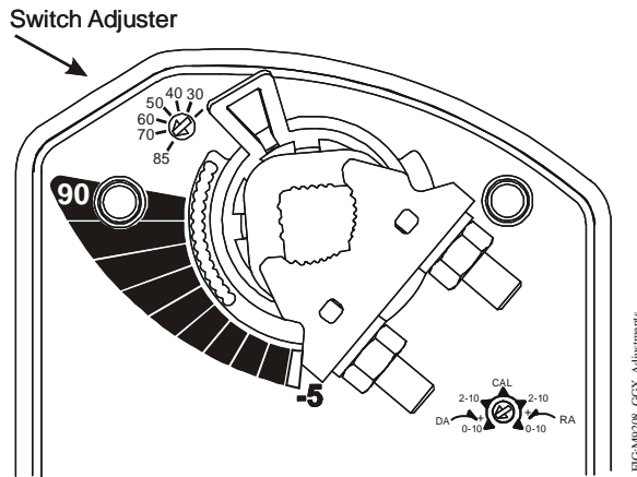
Figure 14: Switch Trip Point Settings
