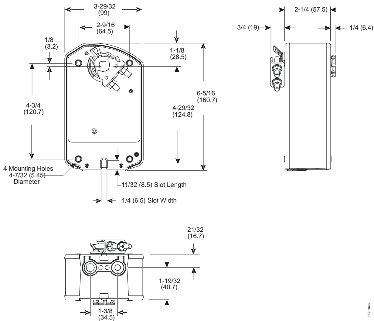
Figure 1: ES70B2(-S) Series Proportional Electric Spring Return Actuator Dimensions, in. (mm)
